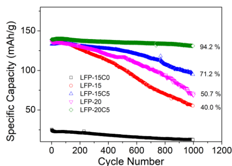
Figure 2 Cycling performance of LFP-15, LFP-20, LFP-15C0, LFP-15C5 and LFP-20C5 under 1 C
