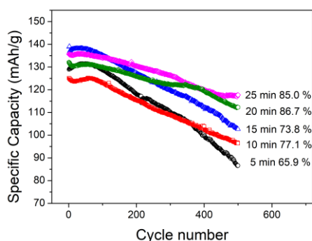
Figure 1 Cycling performance of LFP samples prepared under different reaction time with 2.5 wt% C under 1 C
